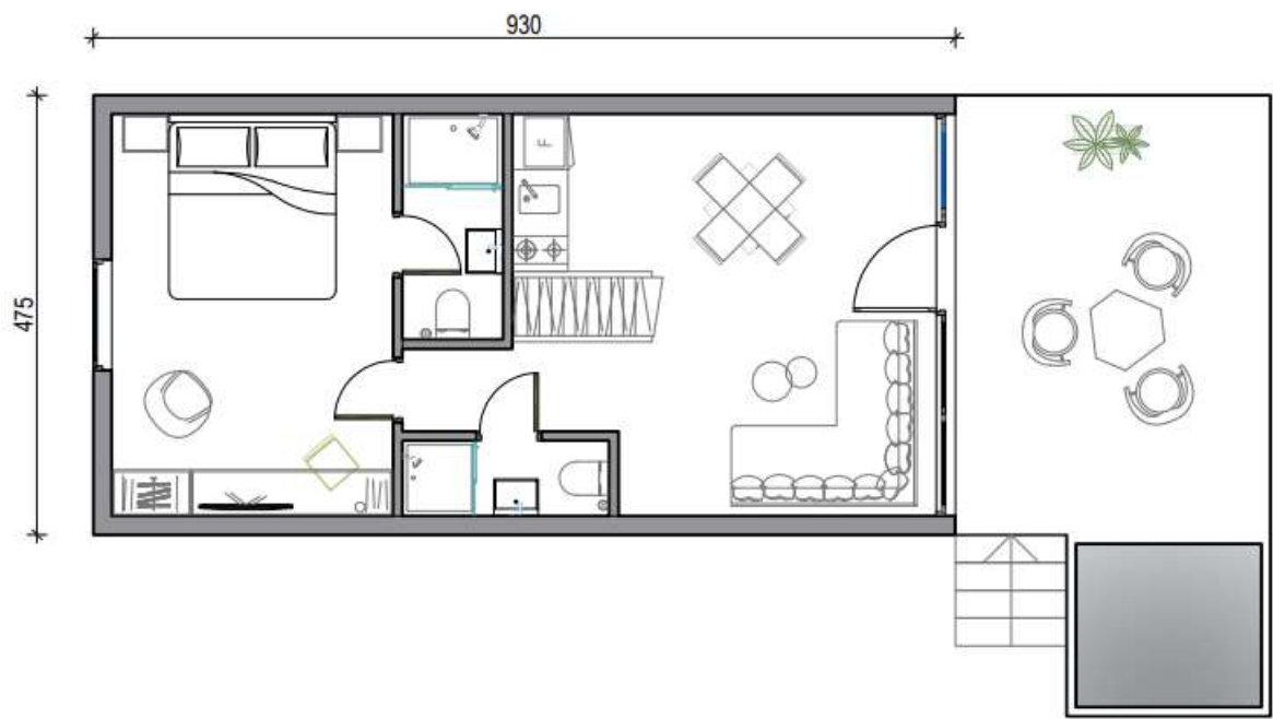
Layout 1. floor
